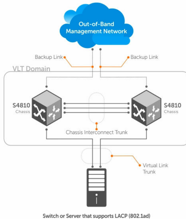
Figure 118. VLT on Switches
